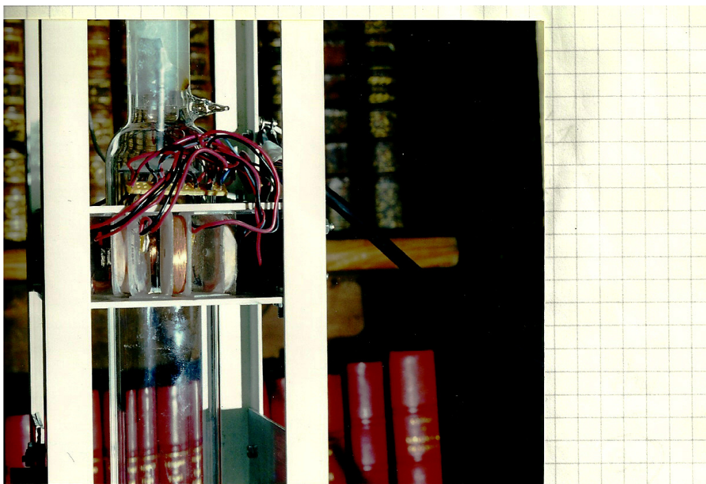
The coils and the overall experimental device for the straight tube.
